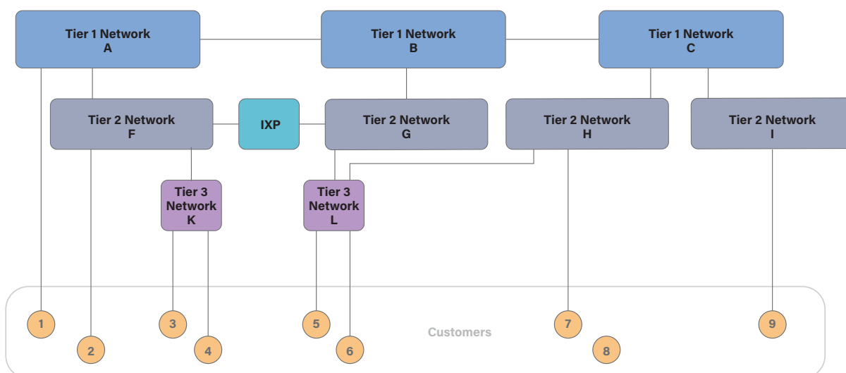
Diagram 1: High Level Topology of Public Internet
